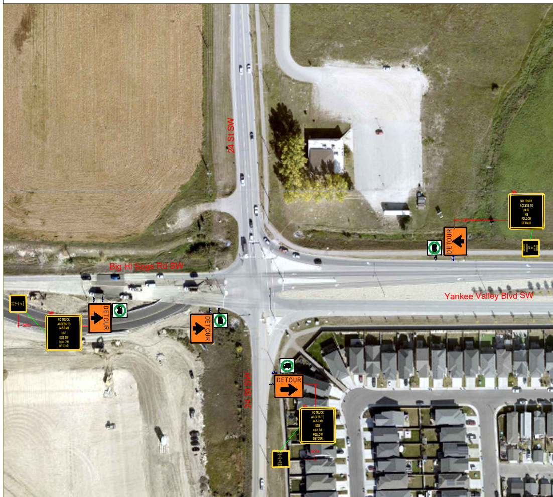
DETAIL 3
