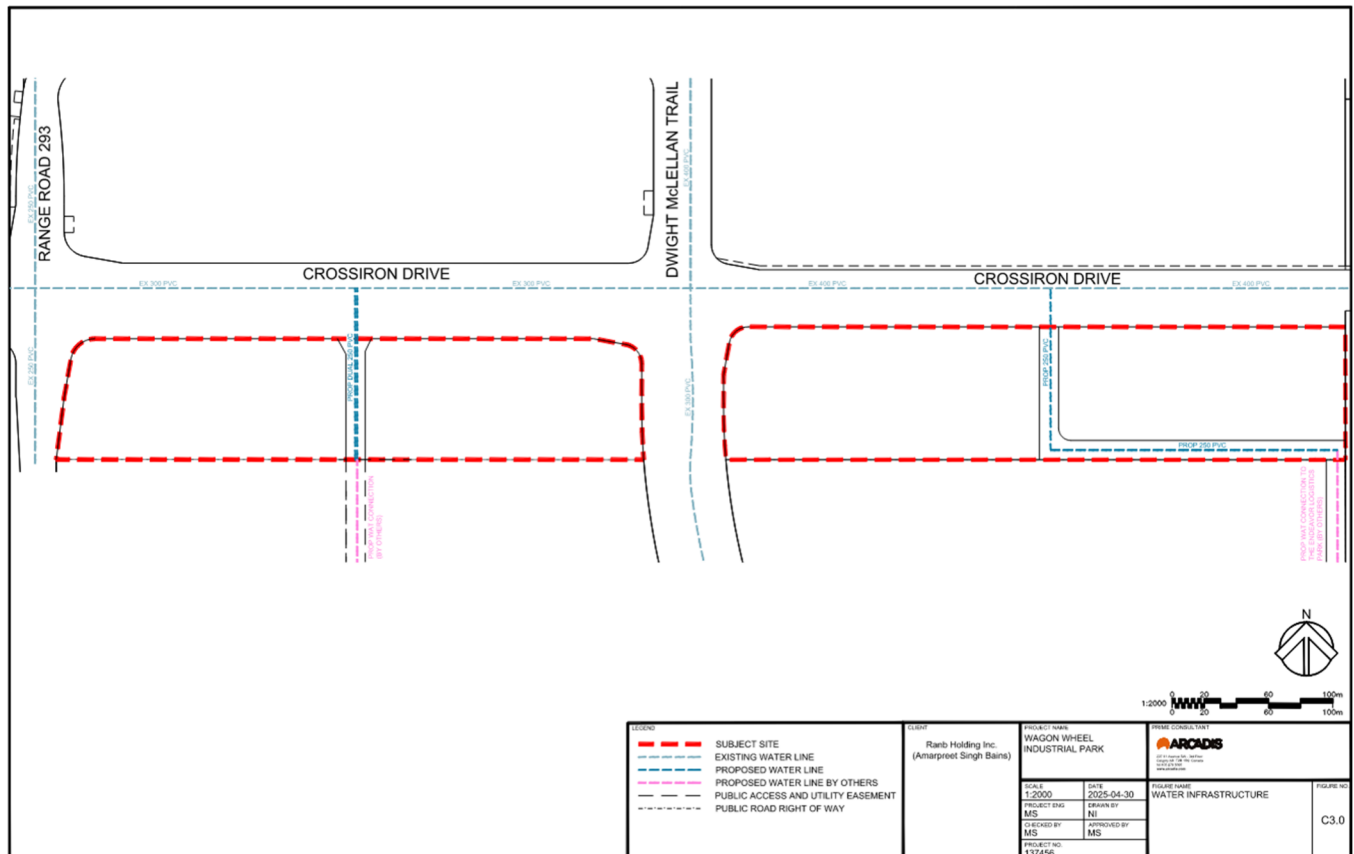
Figure 12: Water Servicing Plan
