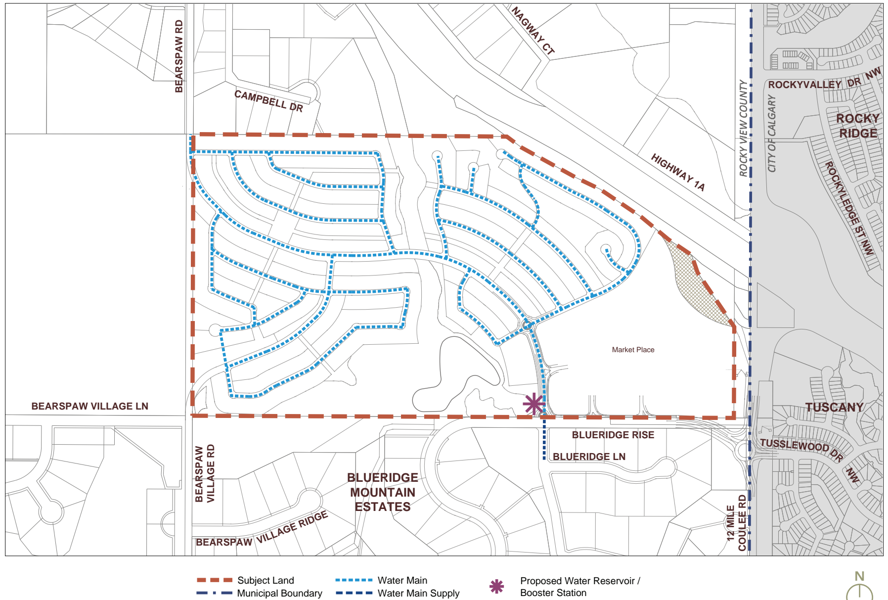
Figure 21 - Internal Water Servicing Plan
